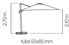
tube 55x85 mm
