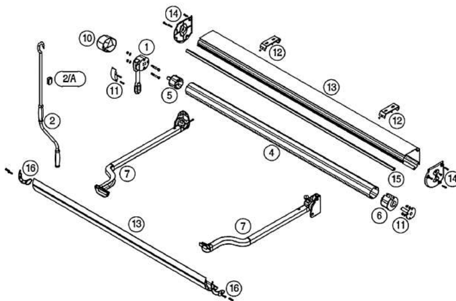
Microbox despiece
