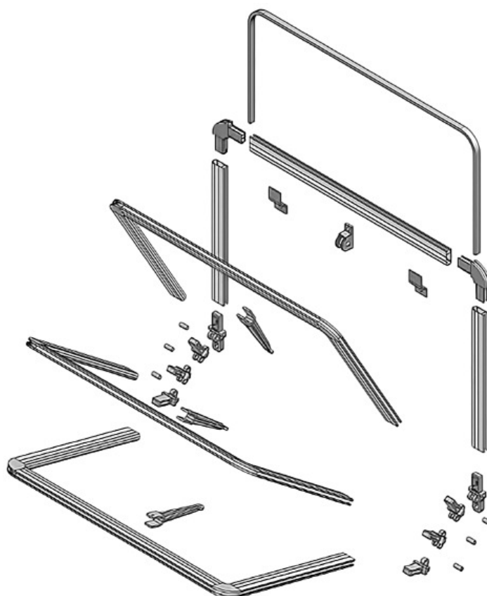
Capota despiece
