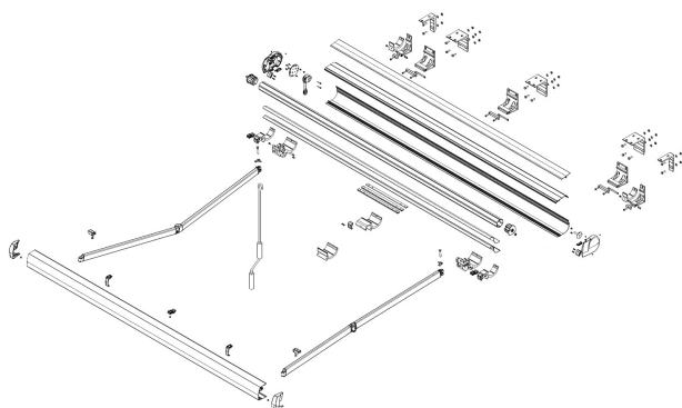
Armony Plus despiece
