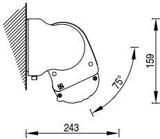
Montaje a pared 75° 75° wall installation
