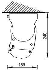
Montaje a techo 90° 90° ceiling installation
